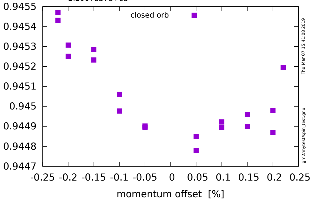
Horizontal tune vs momentum 2.2907837e+05
