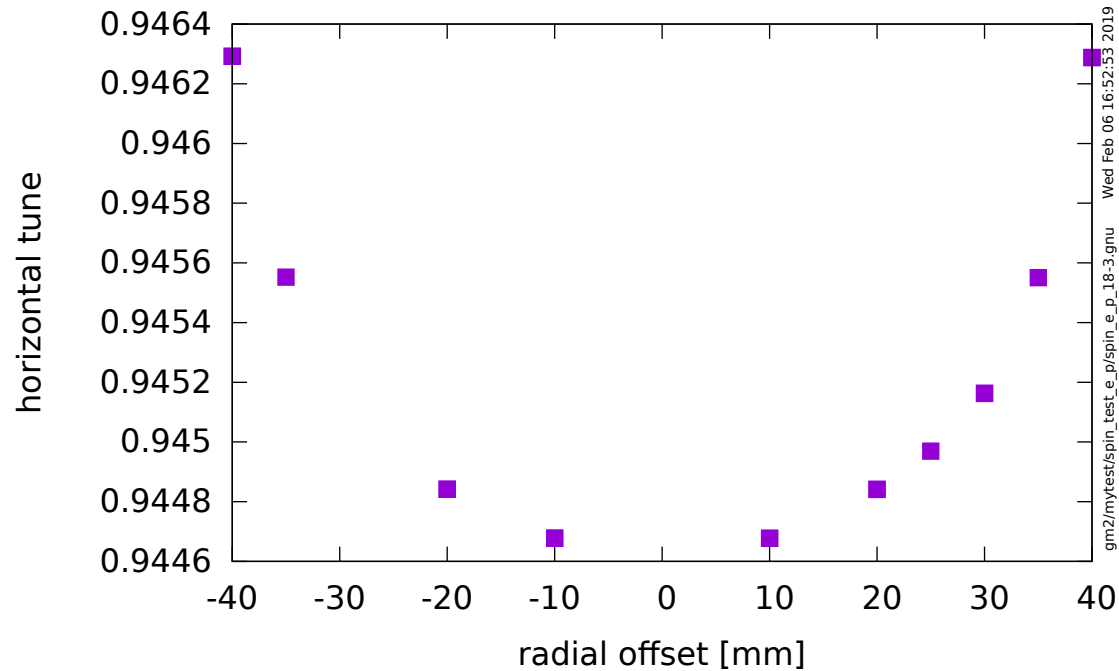
Horizontal tune vs amplitude
